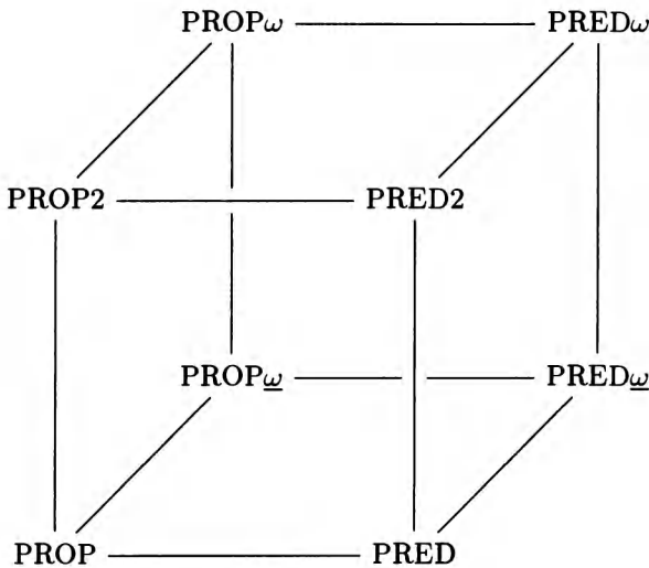
Fig. 3. The logic-cube.
